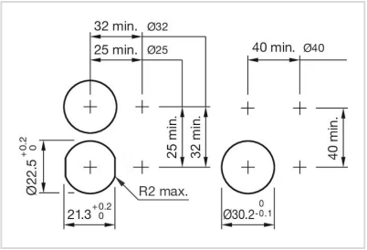
Dimension drawings:
